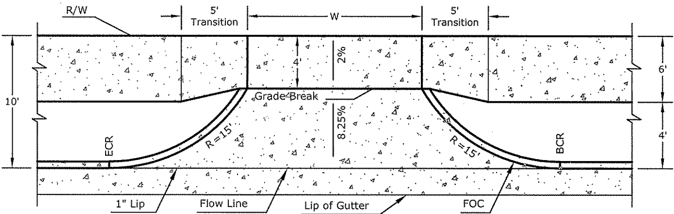
OPTION 3: 6' Sidewalk separated from curb
