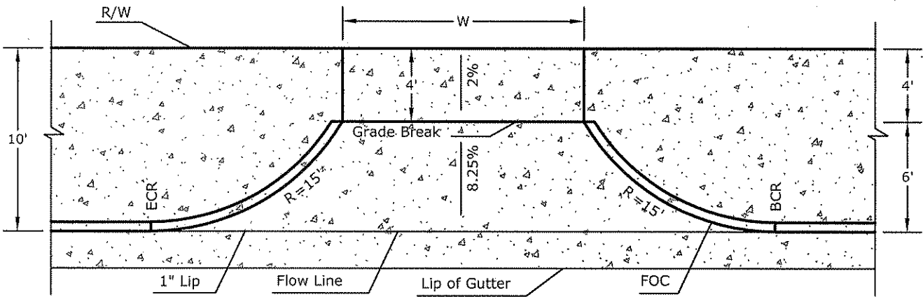
OPTION 1: 10' Sidewalk adjacent to curb
