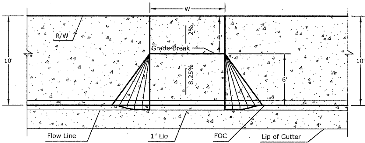
OPTION 4: 10' Sidewalk adjacent to curb
