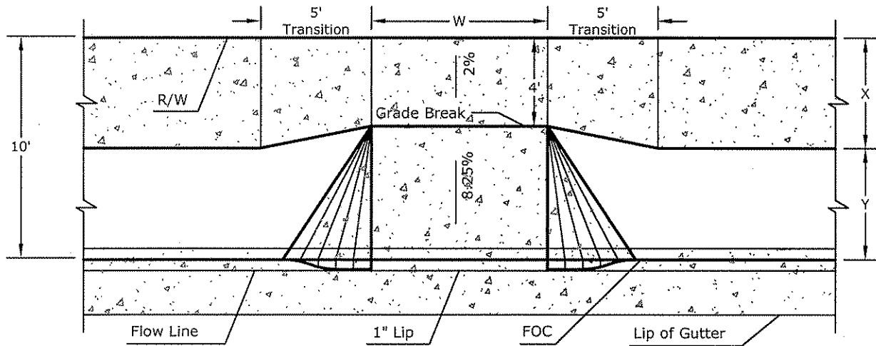
OPTION 5: 5' Sidewalk separated from curb
