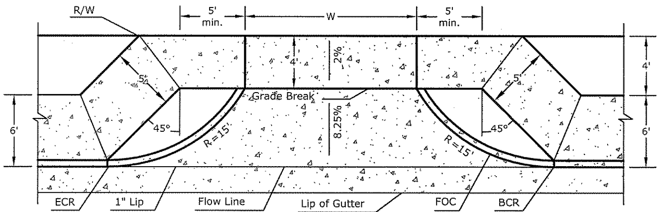
OPTION 2: 6' Sidewalk adjacent to curb
